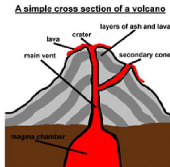
Diagram of a volcano.
